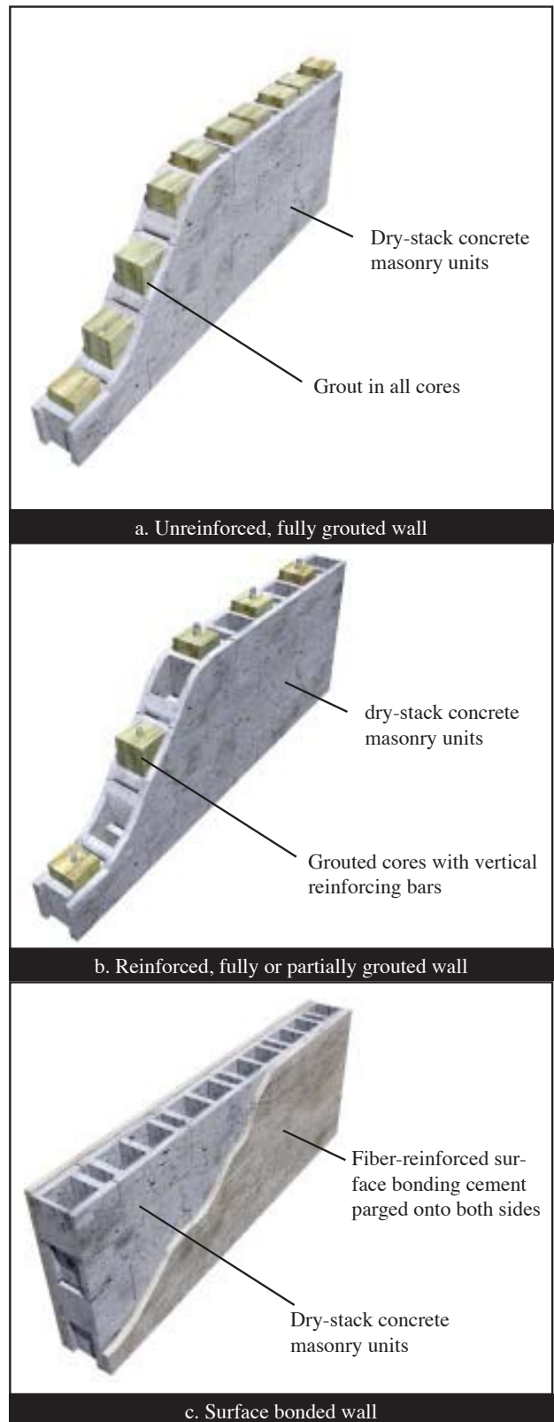
Figure 2—Basic Dry-Stack Masonry Wall Types
