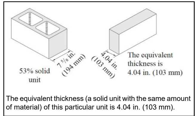
Figure 1—Equivalent Thickness
