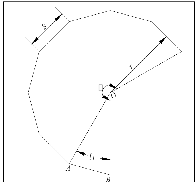
Figure 1—Plan View of Radial Wall Laid in Stack Bond (Regular Polygon)
