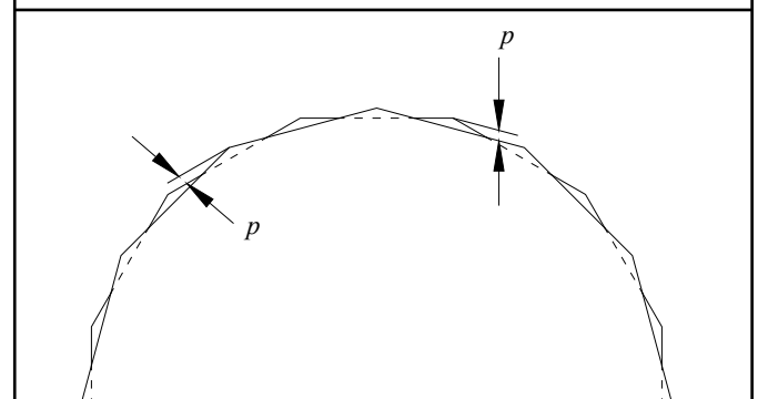
Figure 2—Plan View of Projections in Radial Wall as a Result of Running Bond
