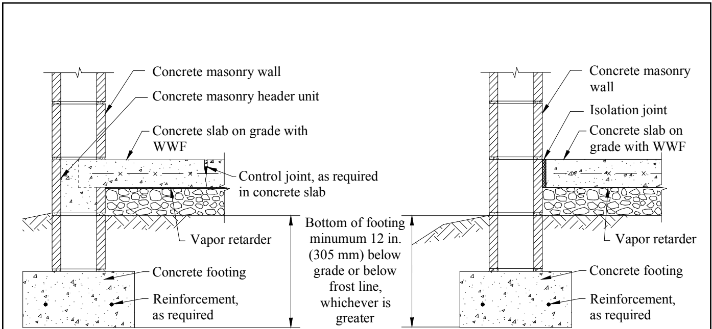
Figure 5—Slab on Grade Stemwalls with Masonry Above Grade
