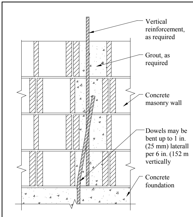
Figure 2—Foundation Dowel Clearance
