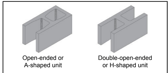
Figure 3—Examples of Unit Shapes that Accommodate Reinforcement
