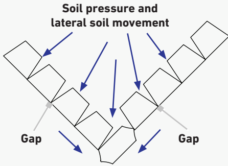
Figure 14.1 | Wall Corner
