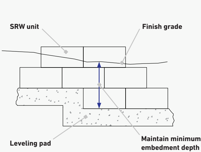
Figure 5.8-1 | Wall Step-Ups
