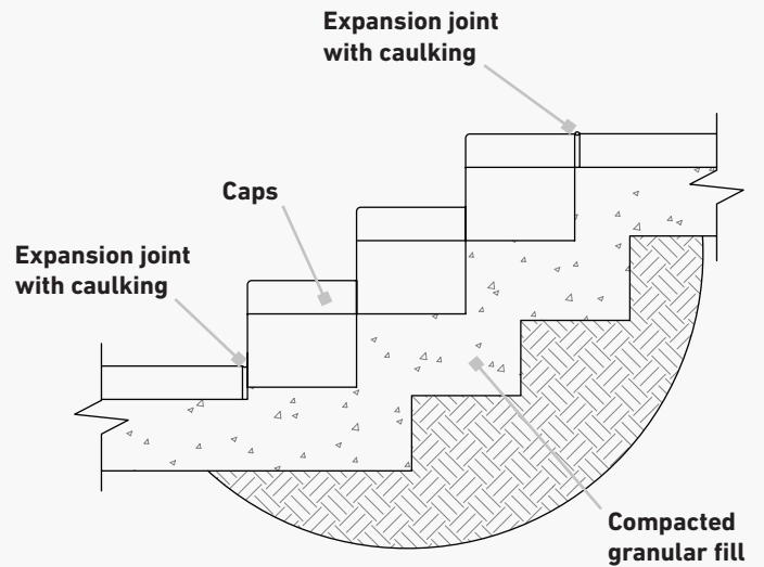
Figure 5.9-1 | Stair Construction
