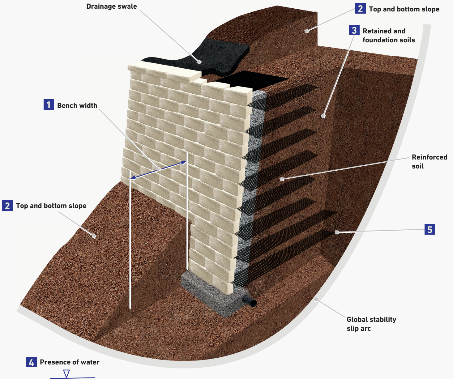
Figure 9 | Global Stability
