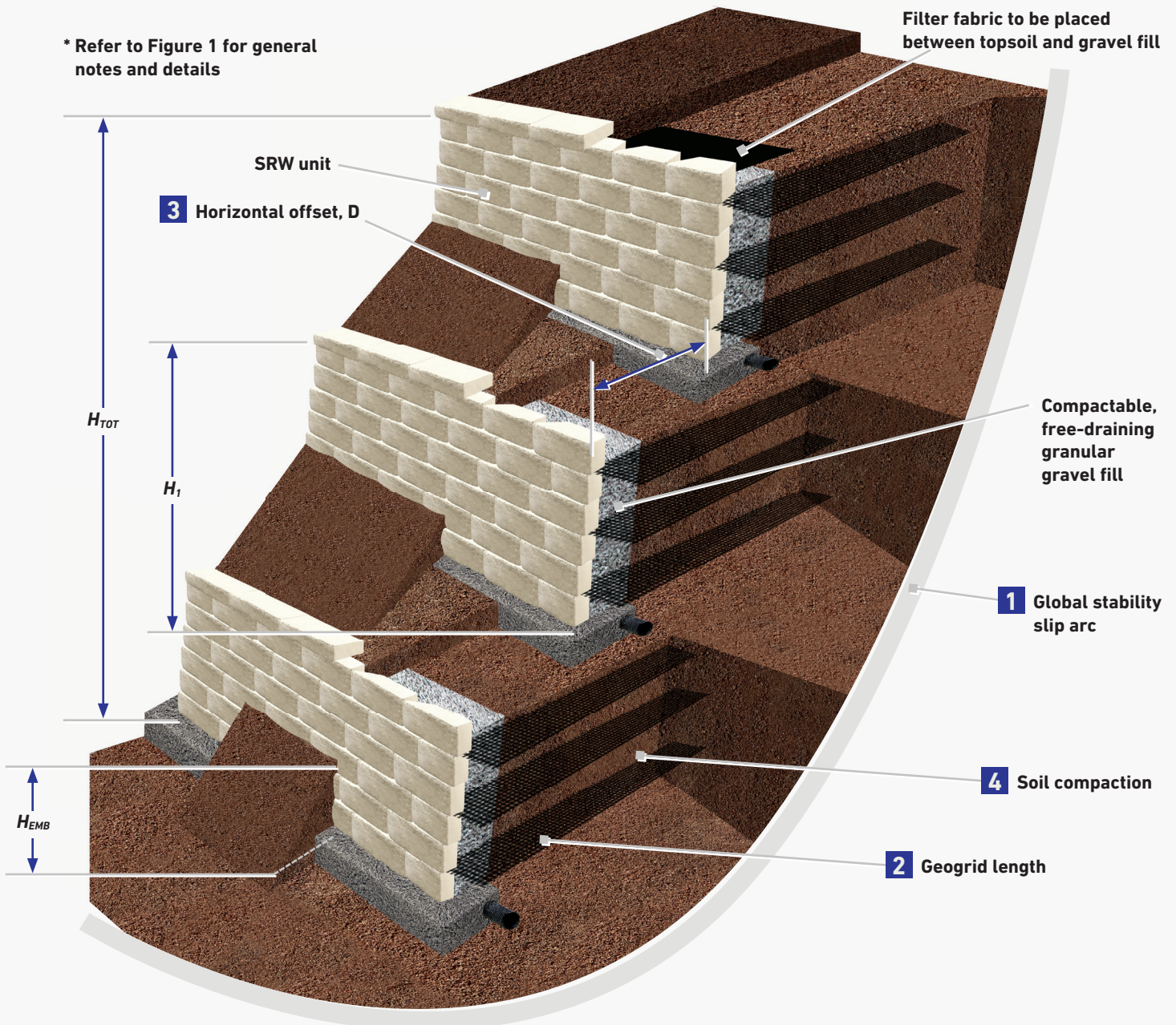
Figure 10 | Terraced Walls
