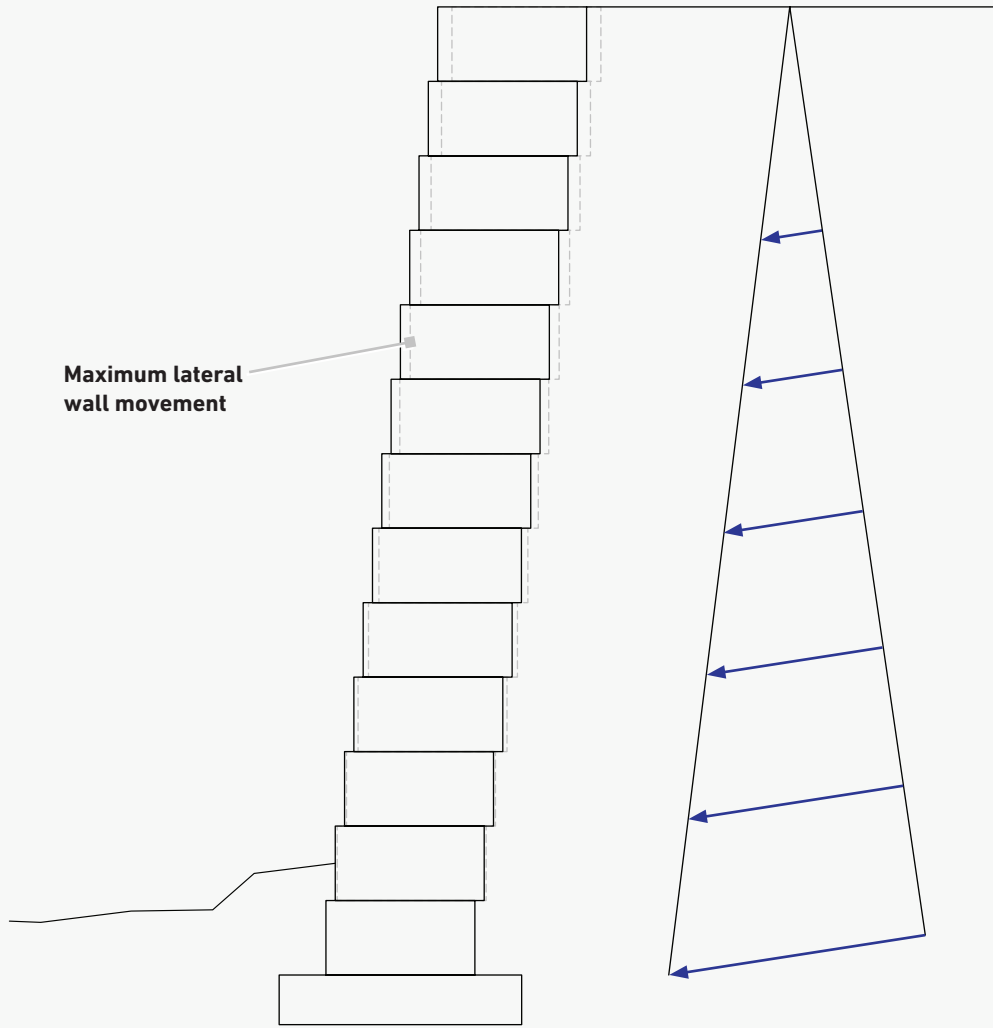
Figure 14.4 | Wall Section
