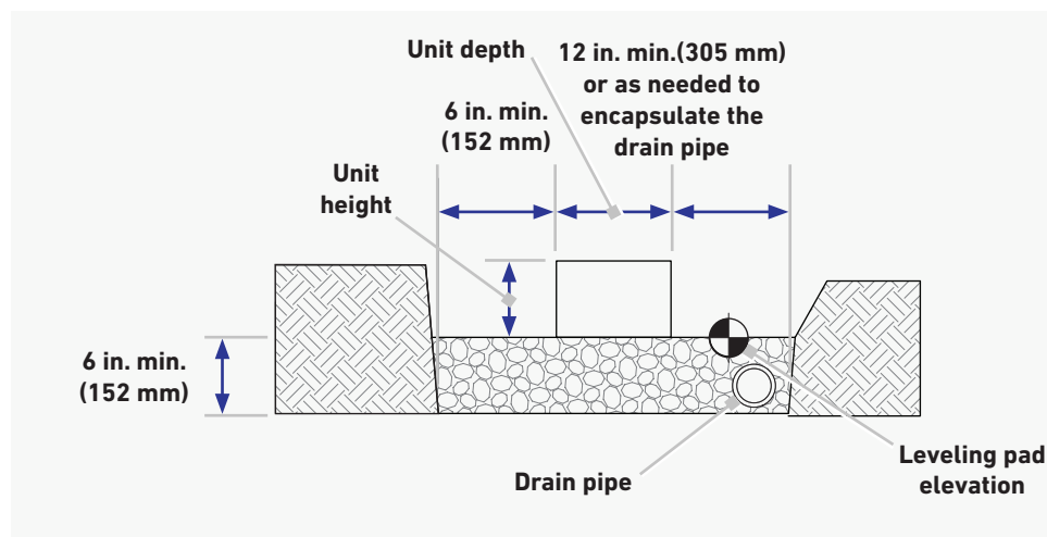
Figure 5.2-1 | Leveling Pad Construction
