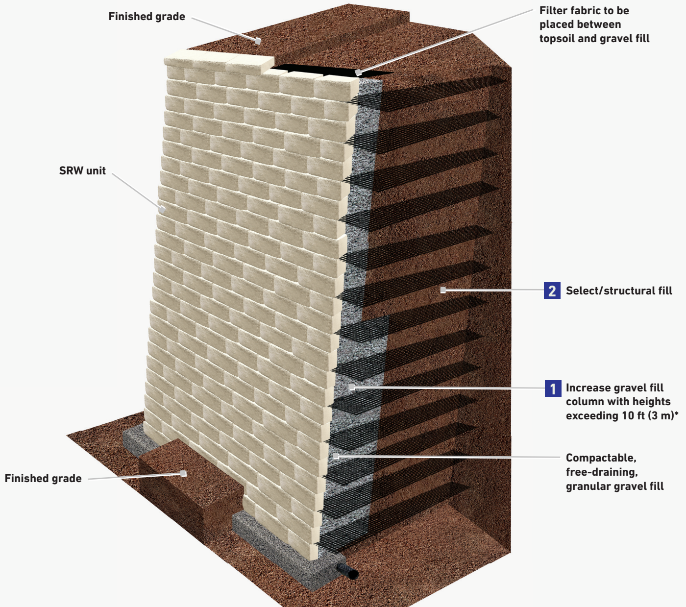
Figure 8 | Tall Walls
