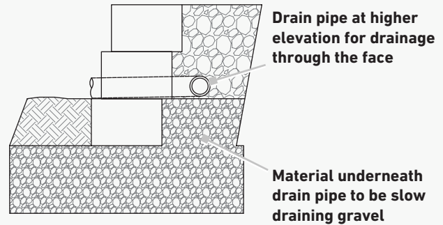
Figure 4.1.2-3 | Optional Drain Pipe Location; Above Base SRW Unit
