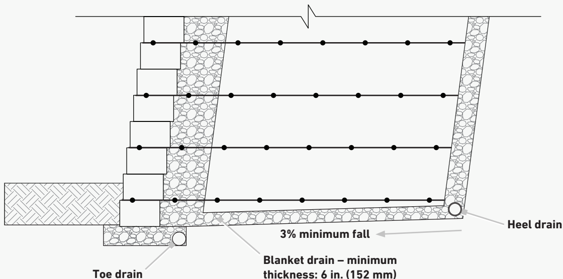
Figure 4.1.2-4 | Heel and Toe Drain Locations
