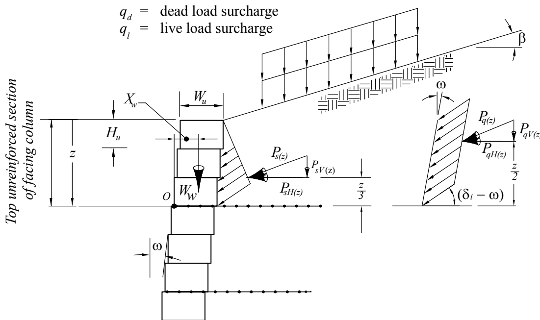
Figure 7-17: Geometry and Forces used to Calculate Crest Toppling
