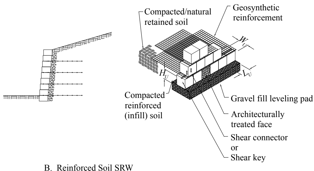
Figure 2-1: Segmental Retaining Wall Systems
