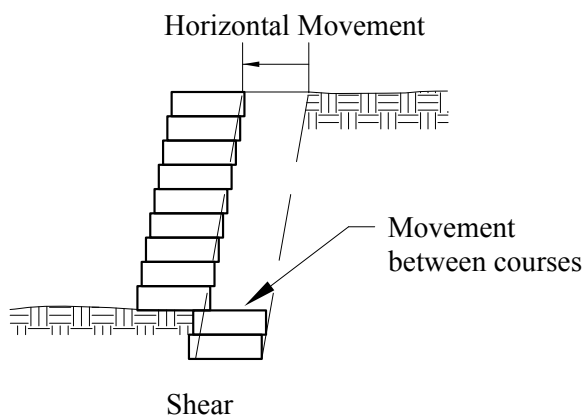
Figure 6-6: Sliding—Main Mode of Failure for Internal Stability
