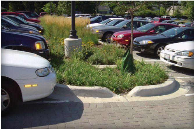
Figure 5. Elmhurst College, Elmhurst, Illinois parking lots uses full infiltration through the soil subgrade with overflows directed through curb inlets into bioretention areas and overflow drains to manage extreme rain events.
