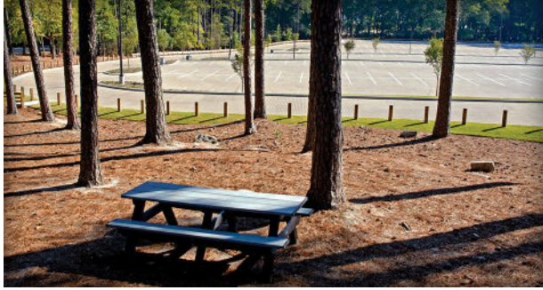
Figure 3. A large PICP parking lot manages an overall site slope of 12% using terraced areas.
