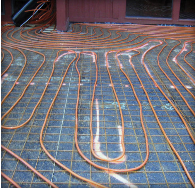
Figure 4. Pipes for a hydronic (liquid) heating system are placed on wire mesh and fastened to it with plastic ties prior to spreading the bedding sand and installing the pavers.
