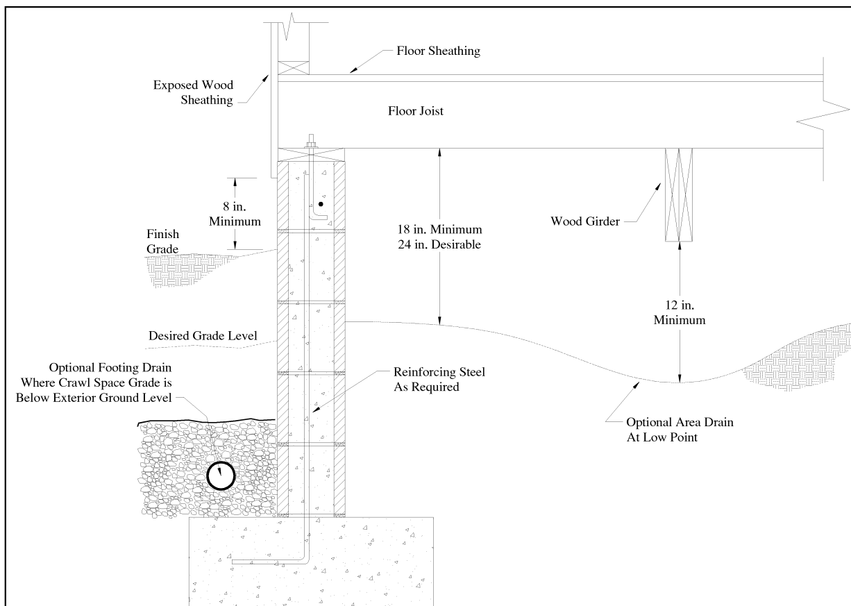
Figure 6-4: Termite Control Measures for Crawl Space Foundations
