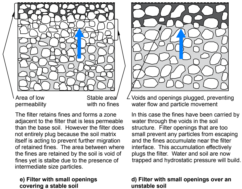
Figure 5.2—Examples of soil and filter subgrades
